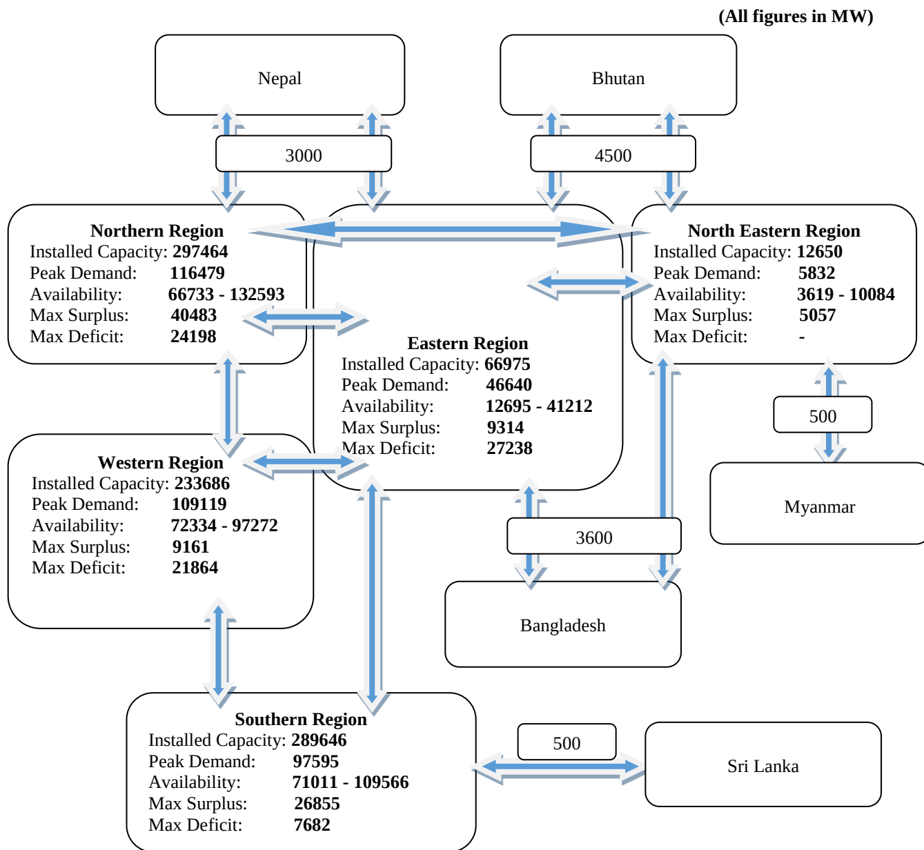
Fig. 8.3: Power scenario of India (including exchange with neighbouring countries) at the end of 2031-32
