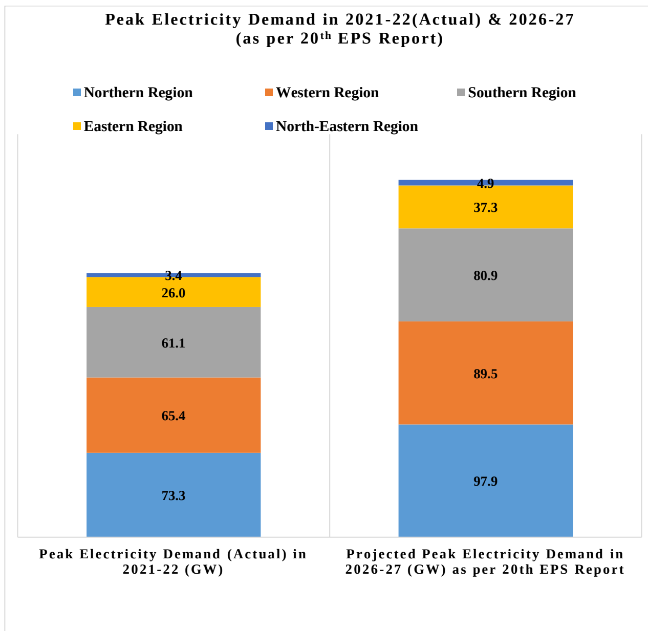
Fig 5.1: Region-wise Peak Electricity Demand in 2021-22 & 2026-27
