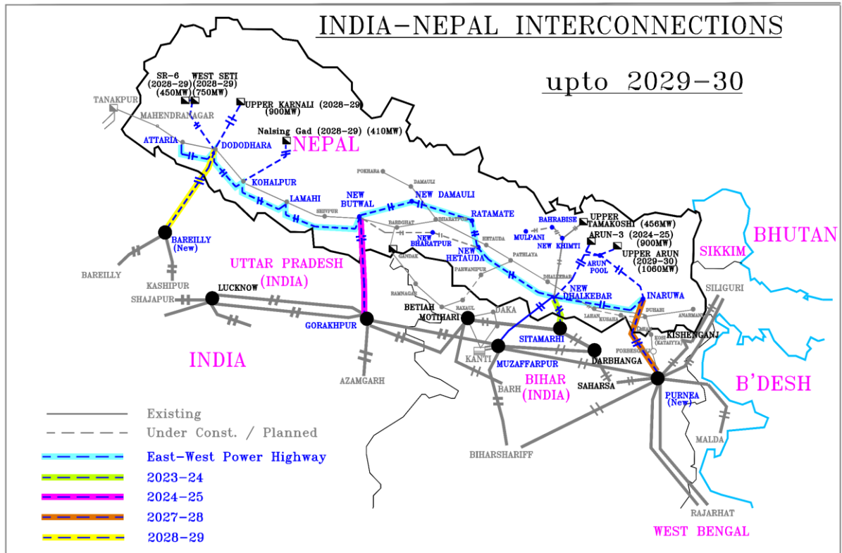
Figure 9.4: India – Nepal Interconnections
