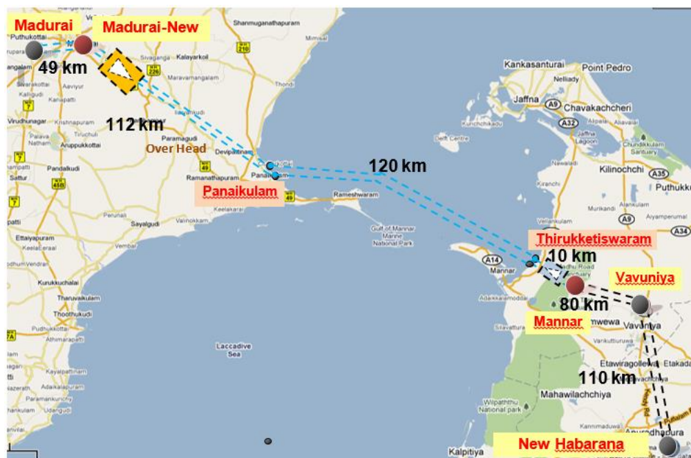
Figure 9.6: India – Sri Lanka Interconnection
